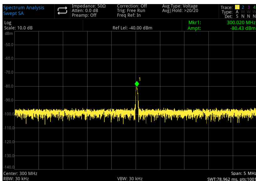
Figure 3-14 Trace Averaging
