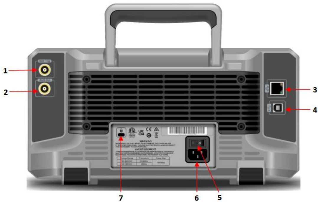
Figure 4 Rear Panel
