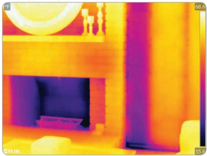
Without MSX
