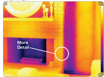
With MSX
