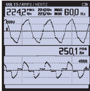
Figure 10C. Flat-topped waveforms.
