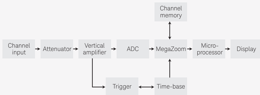
Figure 12. Digitizing oscilloscope architecture.
