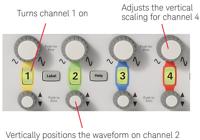
Figure 16. Front panel vertical control section on a Keysight InfiniiVision 2000 X-Series oscilloscope.
