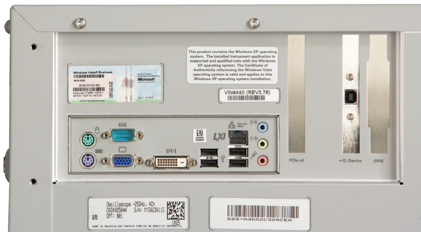
Figure 9. Rear panel on the Keysight Infiniium 9000 Series oscilloscope.
