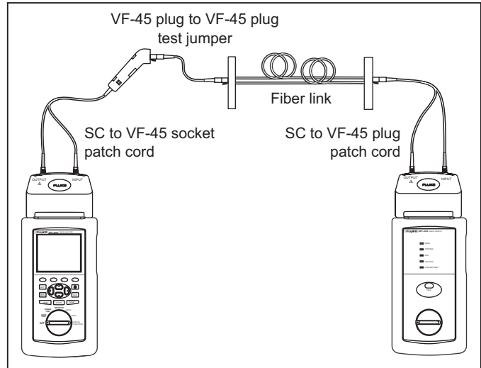
Figure 3. Test Connections
