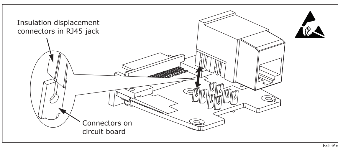
Figure 3. Replacing the RJ45 Jack
