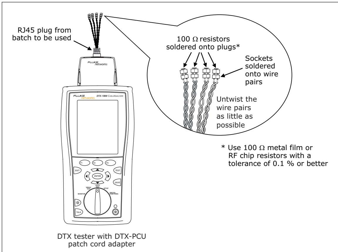
Figure B-1. Pre-qualifying RJ45 Plugs
