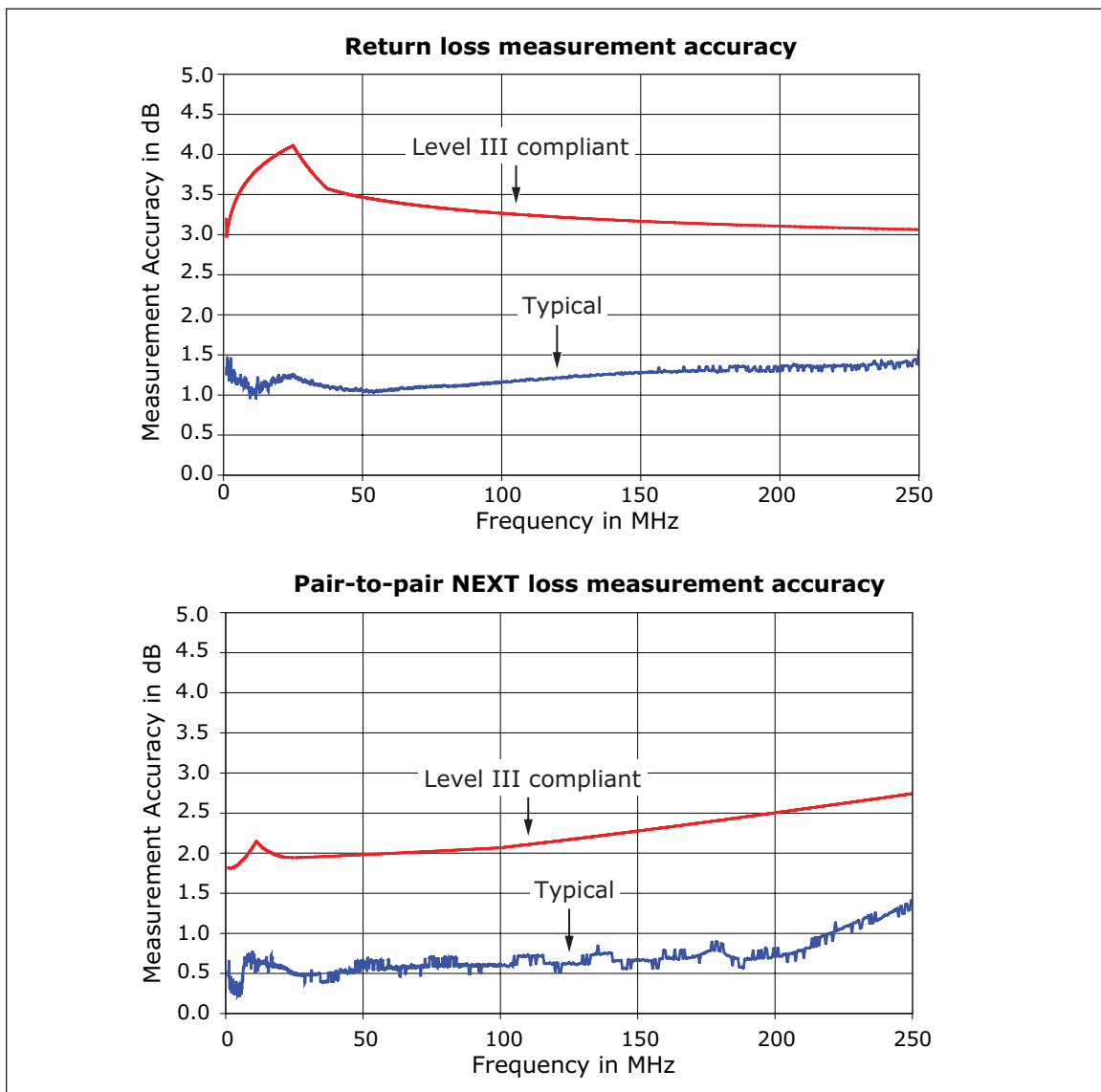
Figure 4. Measurement Accuracy of the DTX-PCU6S Patch Cord Test Configuration
