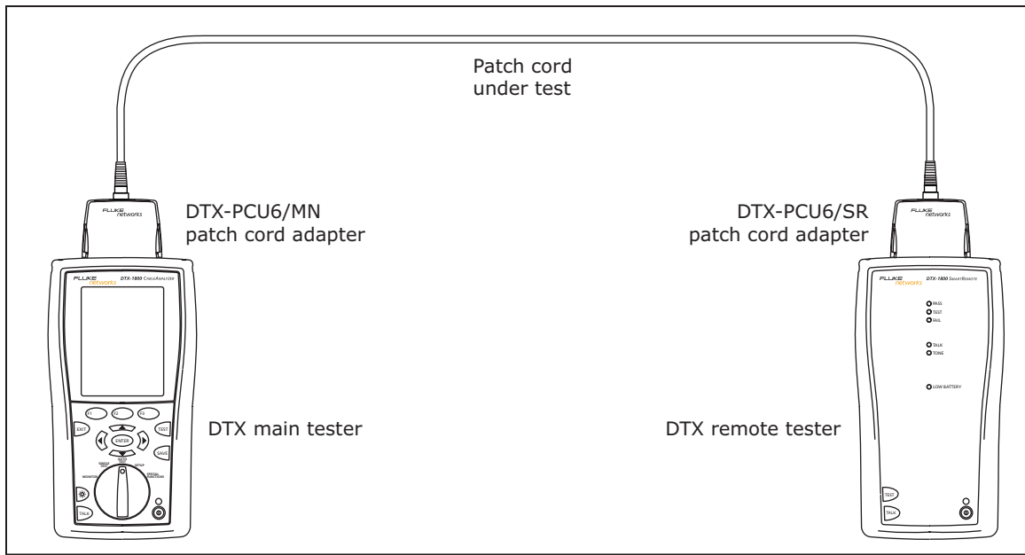
Figure 1. Patch Cord Test Connections
