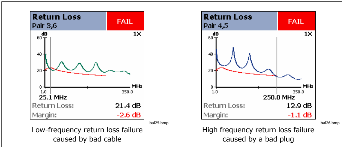
Figure 2. Return Loss Failures at Low and High Frequencies
