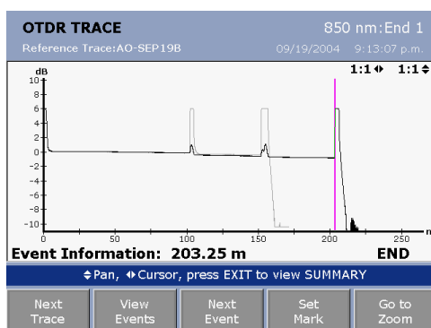
Figure 4: Typical OTDR trace, showing length (203.25 m), a gradual decline in light strength, and two events (connectors, splices or disturbances) at 100 m and 150 m.
