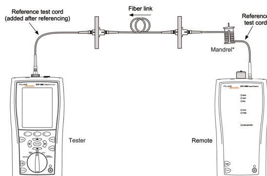
Figure 1: Optical loss measurements use a light source on one end of the link and a power meter on the other. Together they determine the total amount of light lost on a link.
