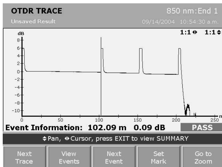
Figure 1. An OTDR trace
