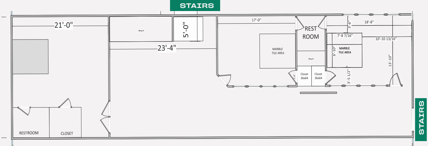
MEZZANINE
