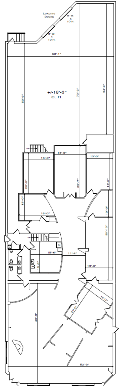
1st floor - 9,975 SF
