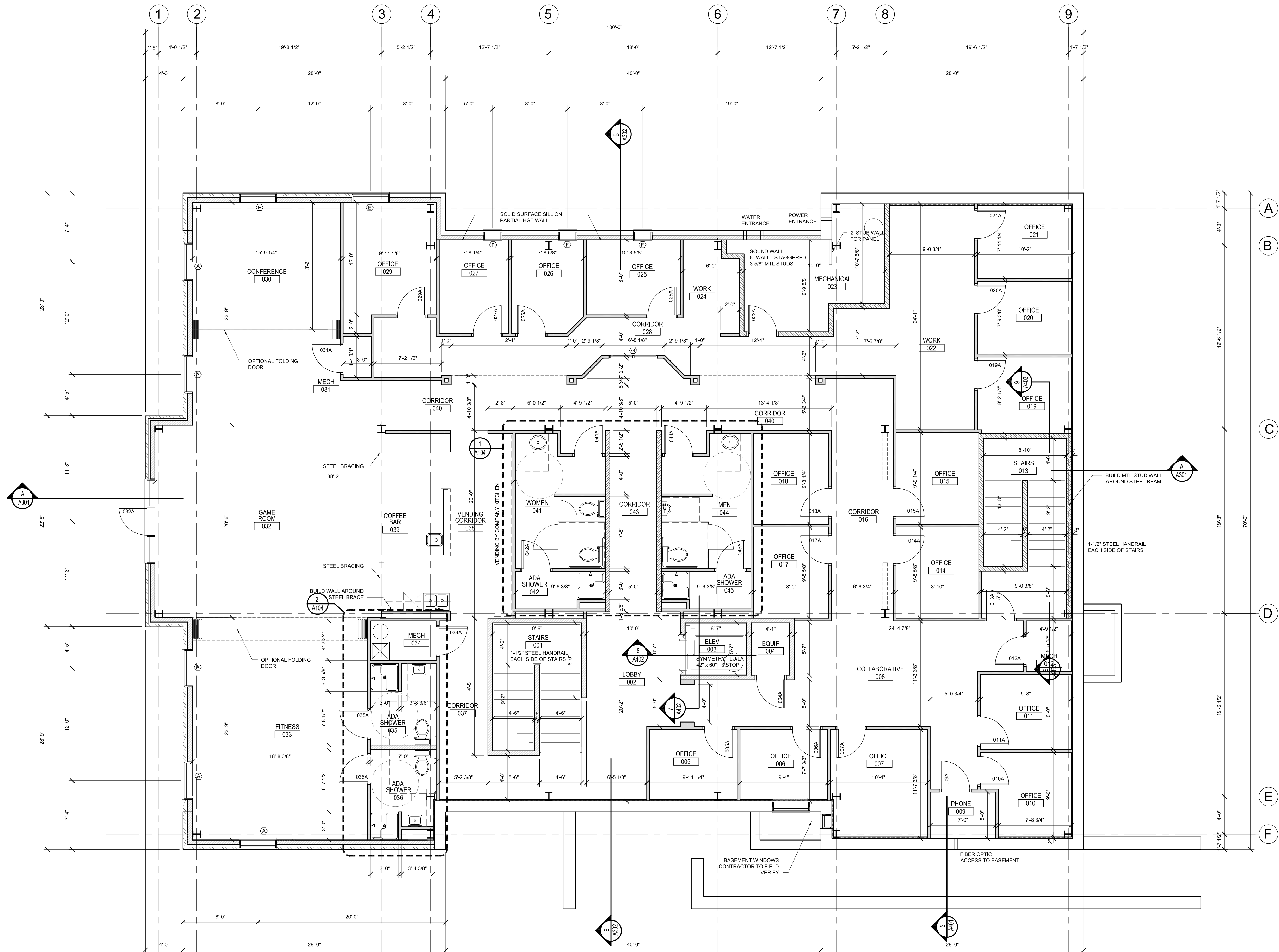
0 BASEMENT INTERIOR PLAN SCALE: 3/16" = 1'-0"
