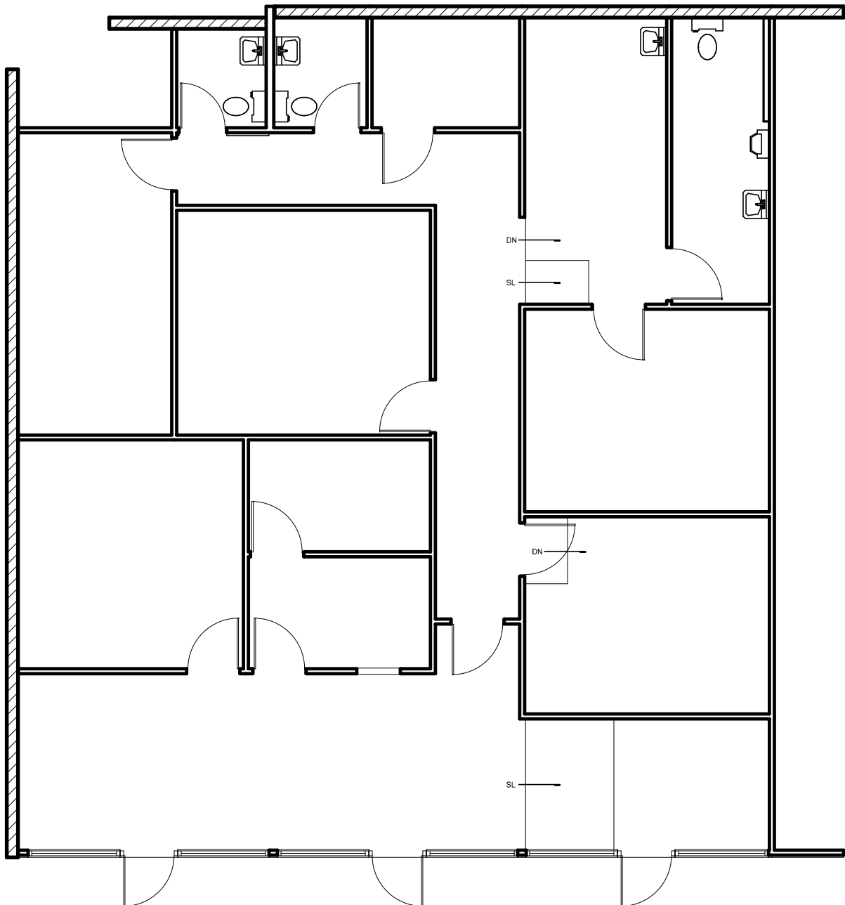
GROUND FLOOR PLAN - SUITE Chino Hills Shopping Center
