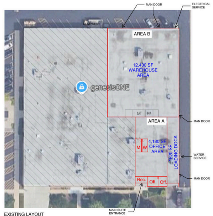
EXISTING LAYOUT
