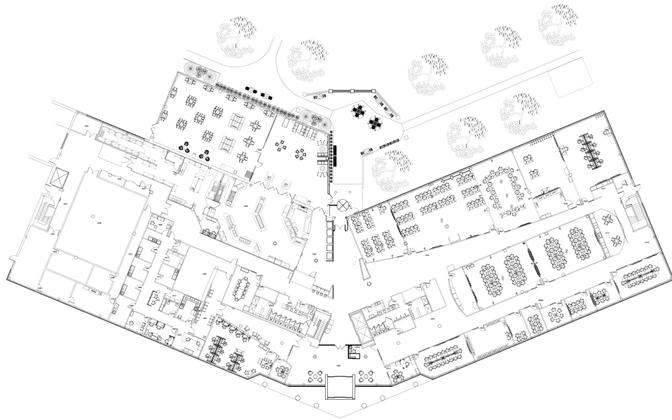
First Floor: 38,400 SF
