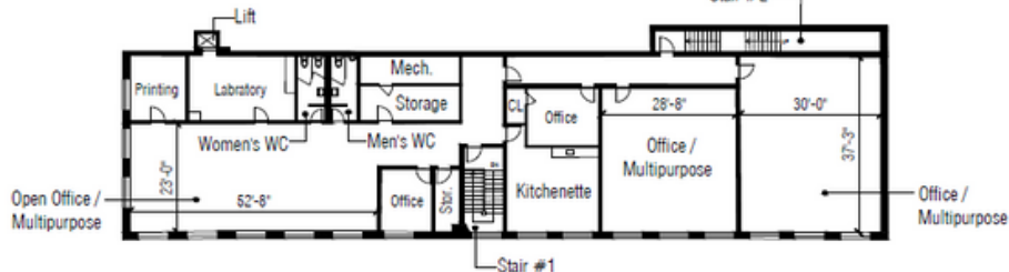
2ND FLOOR
