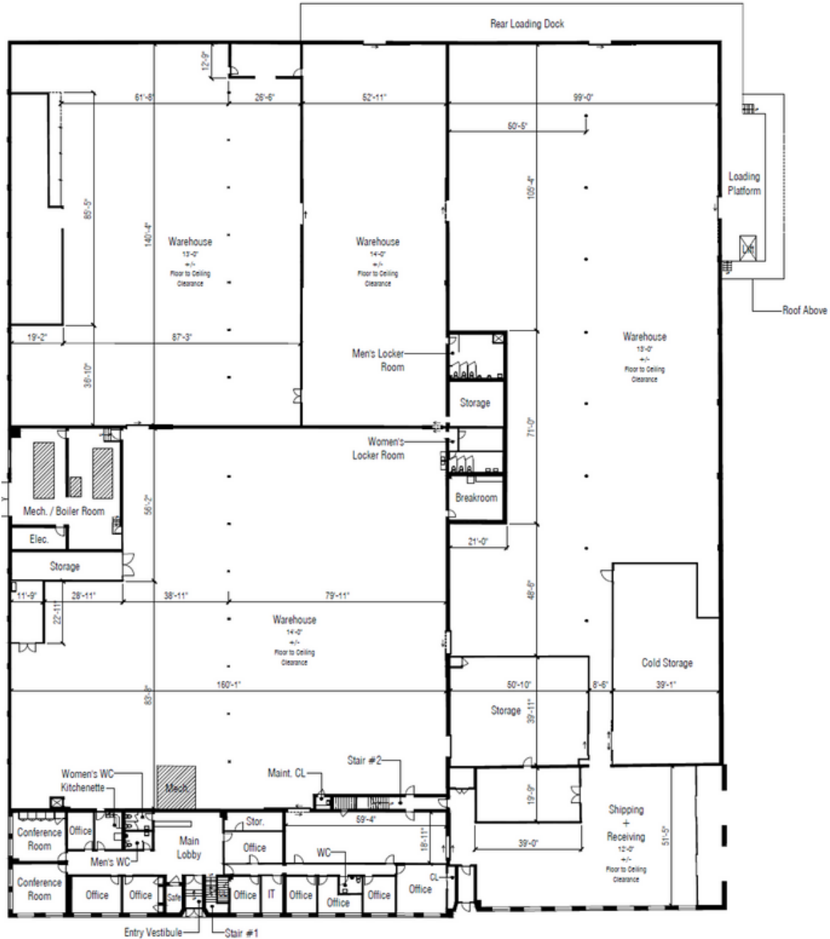
1ST FLOOR
