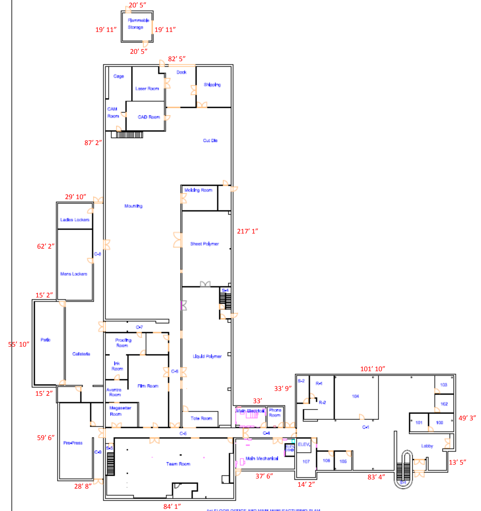
1st FLOOR OFFICE AND MAIN MANUFACTURING PLAN
