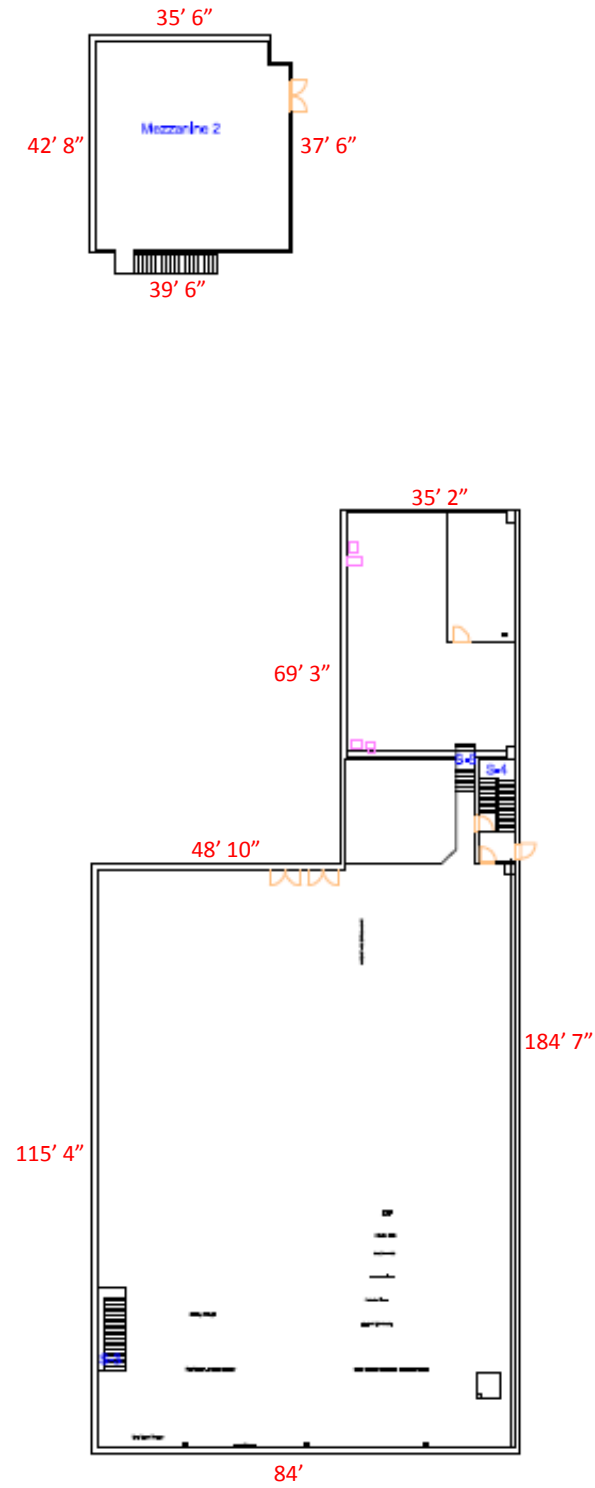
2nd FLOOR OFFICE AND MAIN MANUFACTURING PLAN
