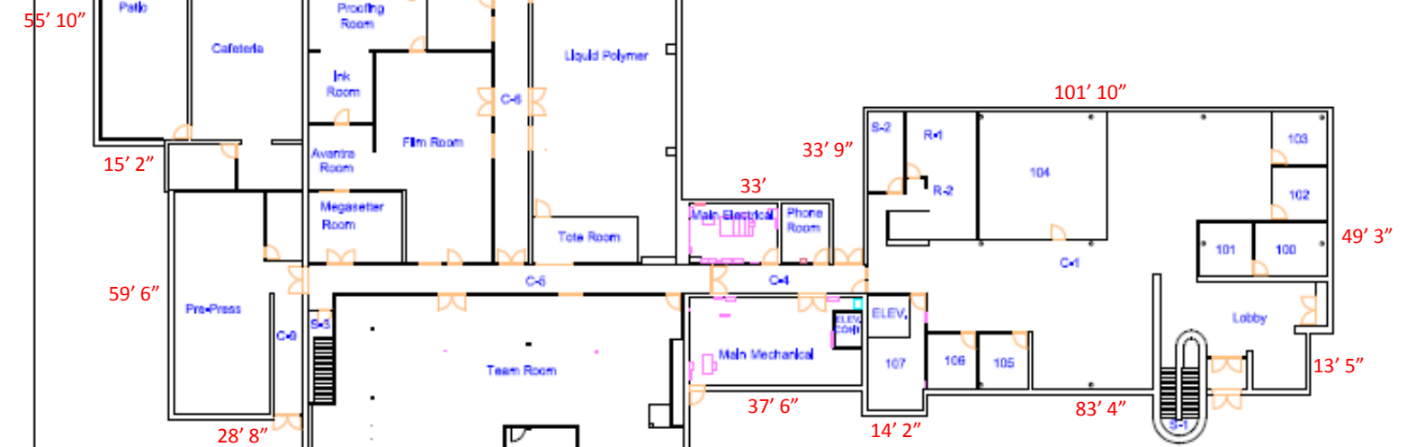
1st FLOOR OFFICE AND MAIN MANUFACTURING PLAN
