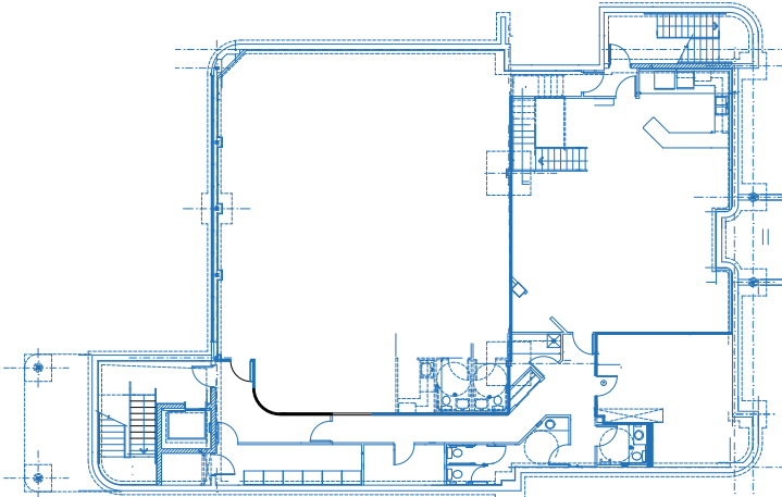
A-2 LOWER LEVEL PLAN
