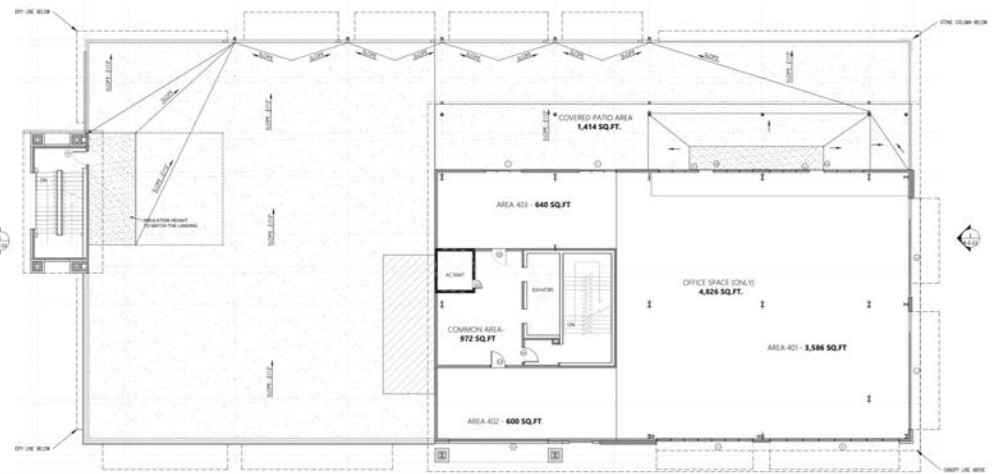
MEZZANINE FLOOR - 4,826 SF
