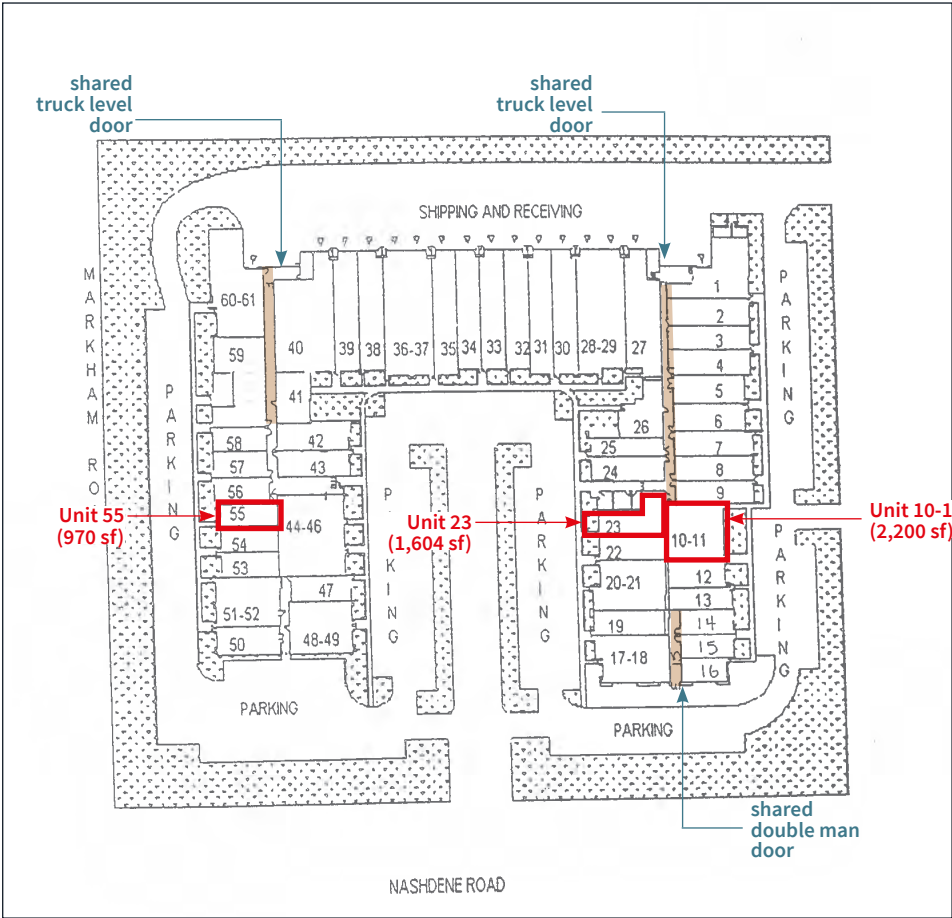
Building Plan
