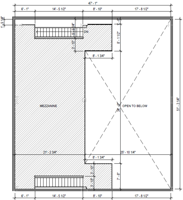
MEZZANINE LEVEL
