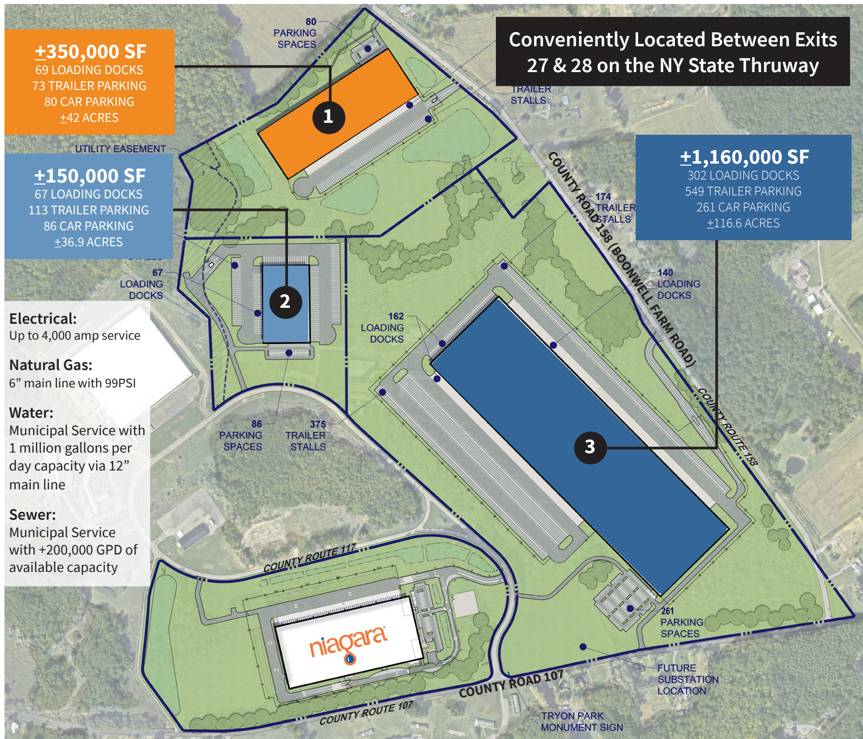
Proposed Site Plan Representative of the Park. Buildings can be tailored to tenant specifications.
