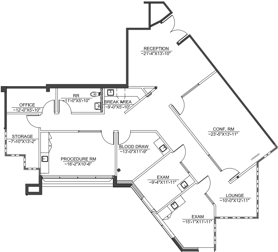
EXISTING MEDICAL BUILD-OUT
