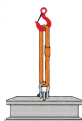
DAMESA Industrial Flat Strap 10000Kg, 6Mx300mm | Orange (116)
