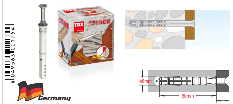
TOX ATTACK 8/60 BOX Nail Wall Plug - 017102221 (052)
