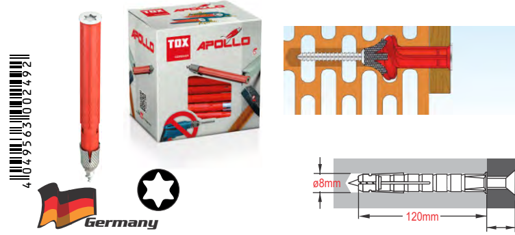
TOX APOLLO 8/120 BOX All-purp. Frame Fixing - 049101151 (101)
