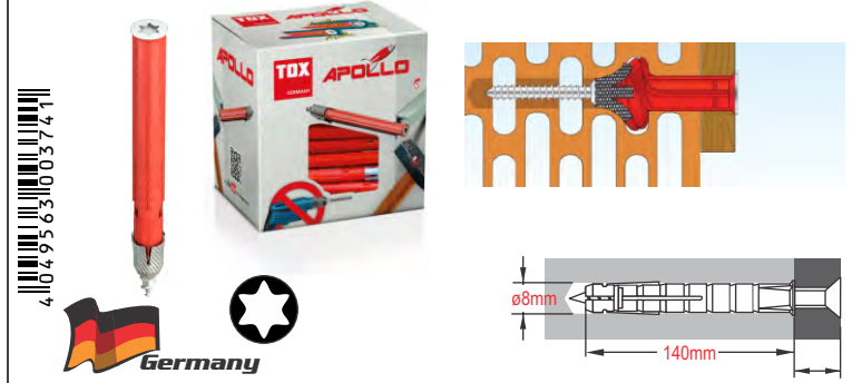
TOX APOLLO 8/140 BOX All-purp. Frame Fixing - 049101161 (102)
