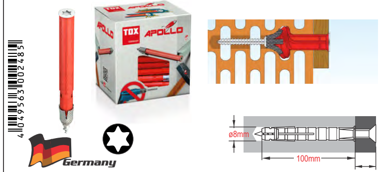
TOX APOLLO 8/100 BOX All-purp. Frame Fixing - 049101141 (100)
