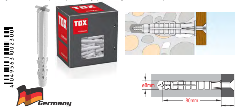
TOX TETRAFIX XL 8/80 BOX All-purp. Framel Plug - 021100101 (061)
