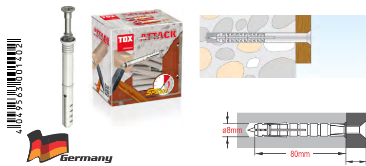
TOX ATTACK 8/80 BOX Nail Wall Plug - 017102231 (053)
