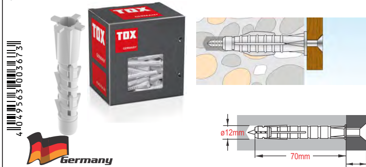
TOX TETRAFIX 12/70 BOX All-purpose Wall Plug - 021100151 (063)
