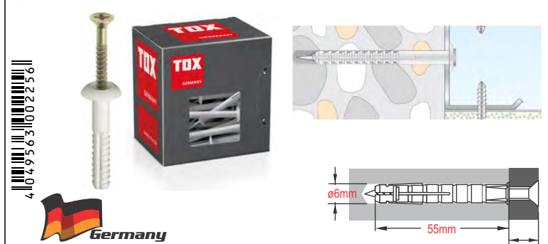
TOX ATTACK METAL 6/55 BOX Hammer fixing - 019102151 (058)
