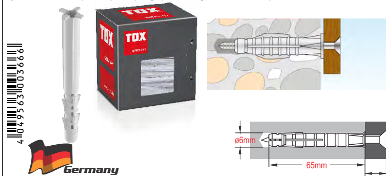
TOX TETRAFIX XL 6/65 BOX All-purp. Frame Plug - 021100051 (064)
