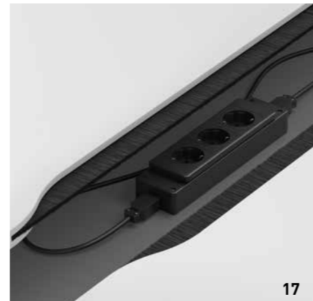
17 | OPEN SLIDING TOP Easy access to the central cable tray and electrics.
