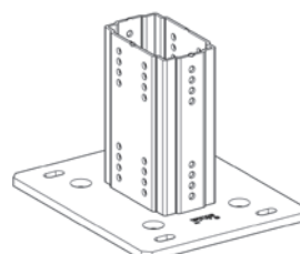
Endefeste WBD F 100/160
