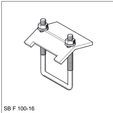
SB F 100-16
