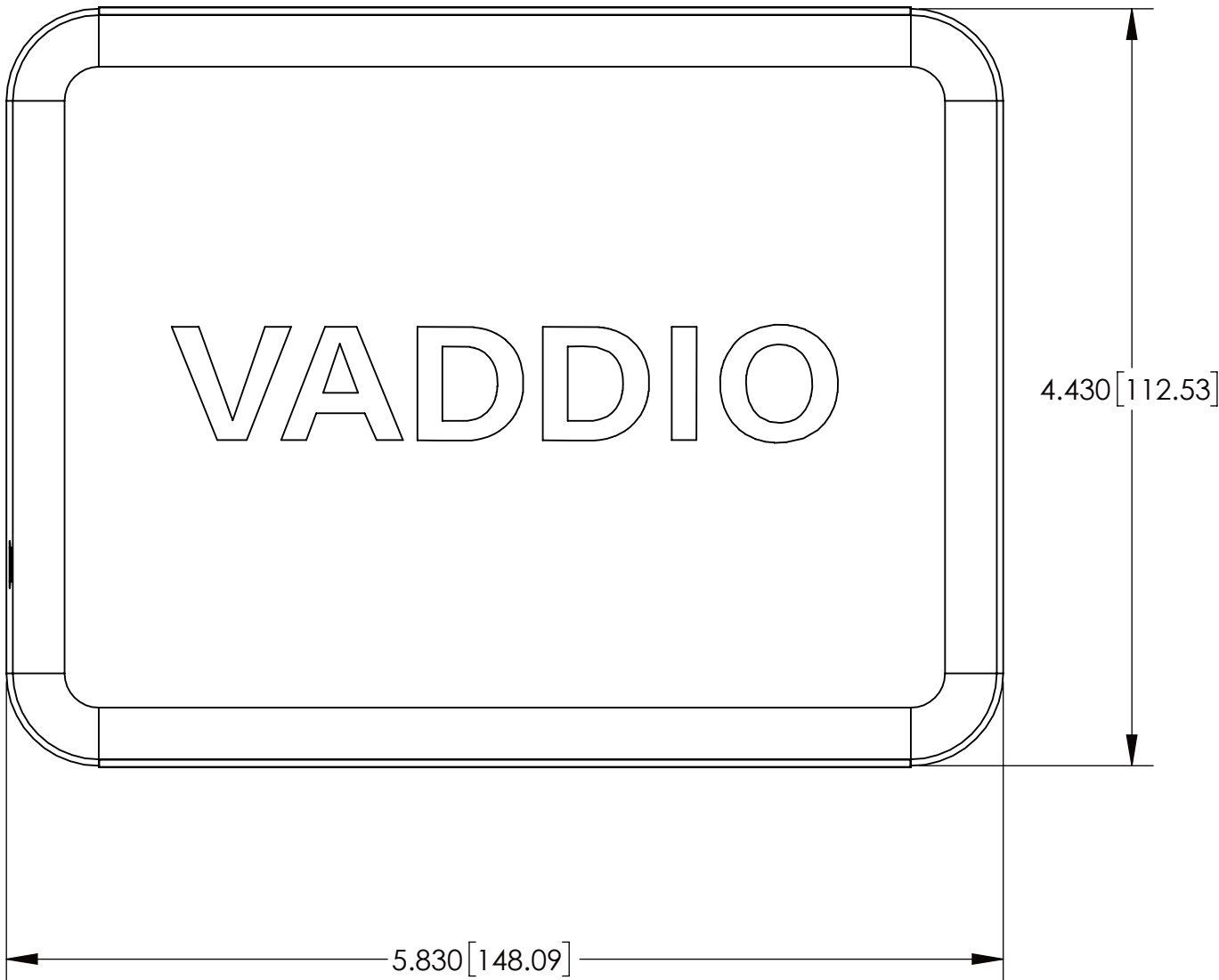
TOP VIEW
