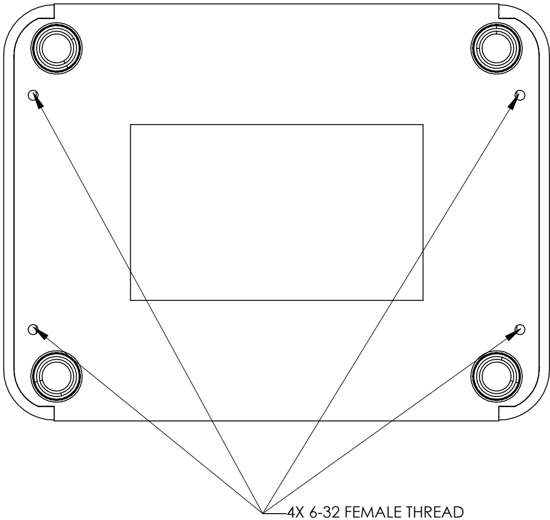
BOTTOM VIEW
