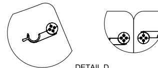
DETAIL D JOINING MULTIPLE TABLES TOGETHER SCALE 1 : 8
