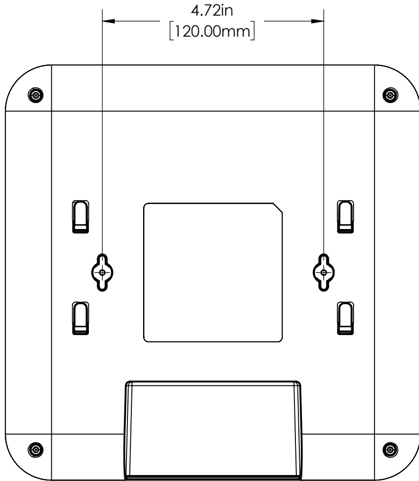
BOTTOM VIEW (W/O MOUNTING BRACKET)
