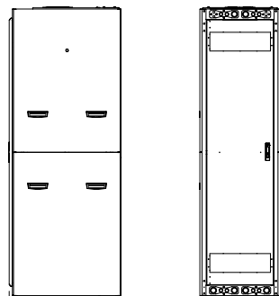
MRK-4431-AV 31.40 OVERALL DEPTH 29.00 USABLE DEPTH
