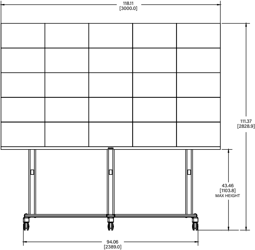
5x5 Mobile Cart Technical Drawing
