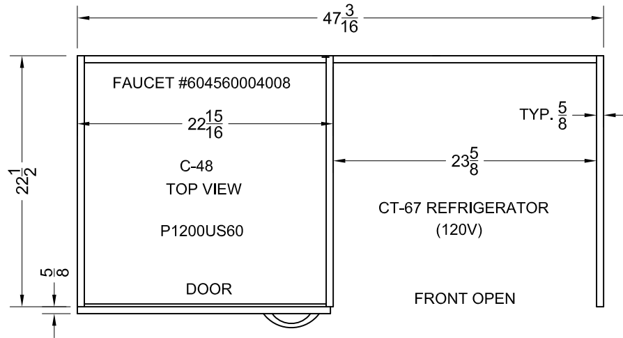
ALL-IN-ONE KITCHEN C-48
