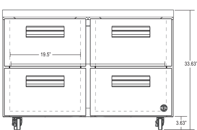
CRMR48-D4 FRONT
