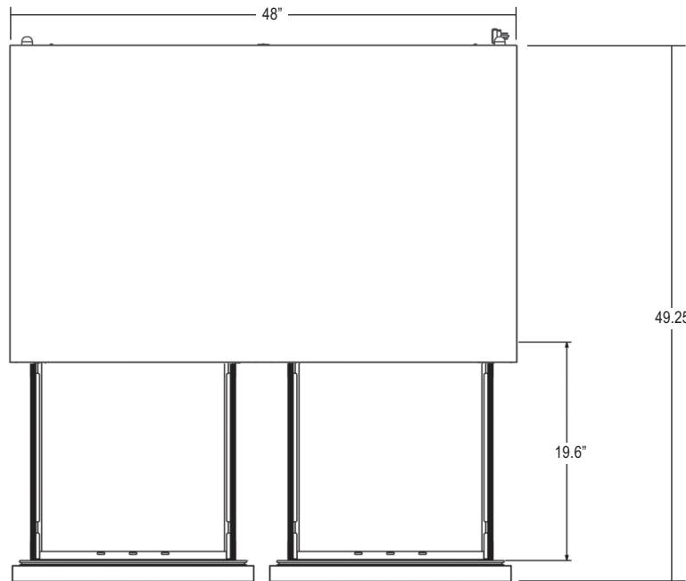
CRMR48-D4 PLAN VIEW
