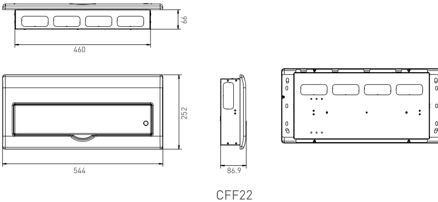
Consumer Unit Knockout Detail per face
