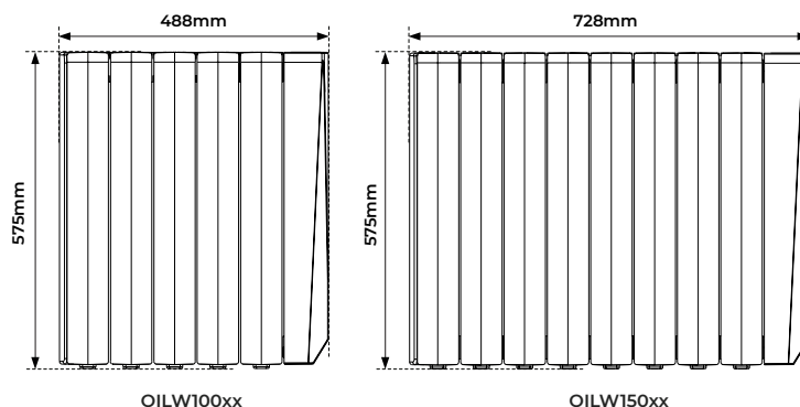
Product Drawing
