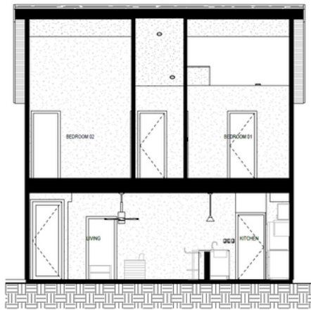
3 BLDG 2 - SECTION 3 SCALE: 1/4" = 1'-0"
