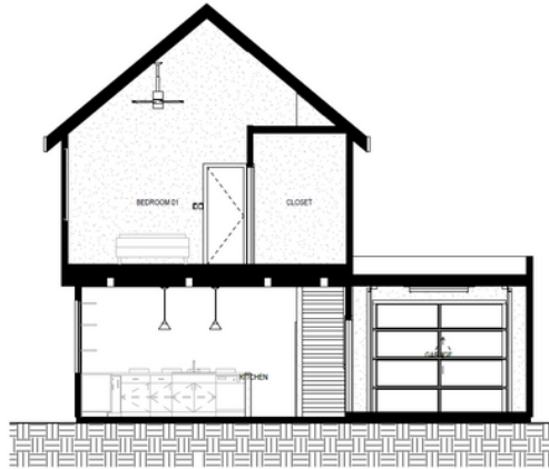
1 BLDG 2 - SECTION 1 SCALE: 1/4" = 1'-0"
