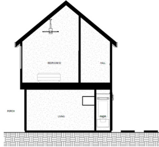
2 BLDG 2 - SECTION 2 SCALE: 1/4" = 1'-0"
