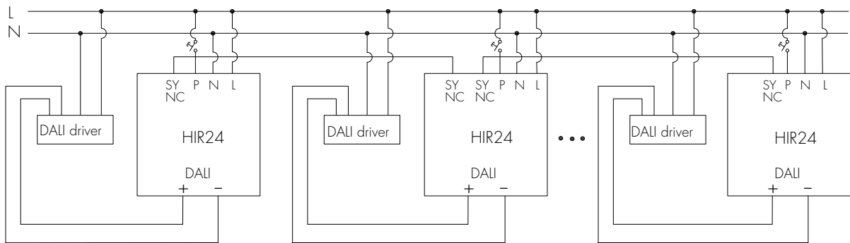
Wiring Diagram
