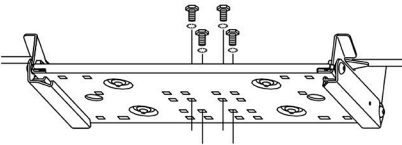
Single mount non-through-bolt applications, including Style 1 "Levelock" 4 Hex head bolts & lock washers.
