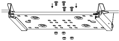
Single mount through-bolt applications 4 Carriage bolts & lock nuts.
