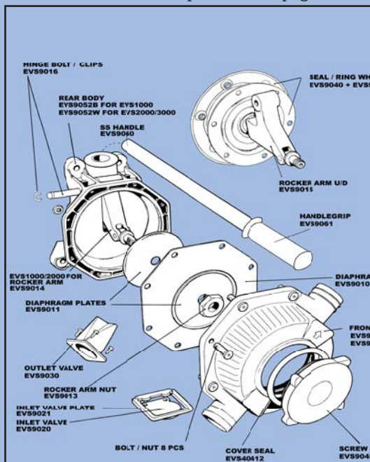
EVS1000/2000/3000 Exploded - See page 9.
