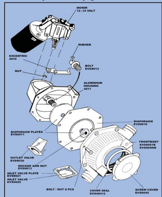
EVS4008 Exploded - See page 10.
