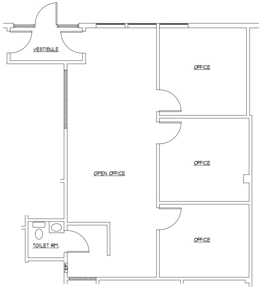
EXISTING FLOOR PLAN - SUITE 1130 SCALE 1/8" = 1'-0" 929 SF
