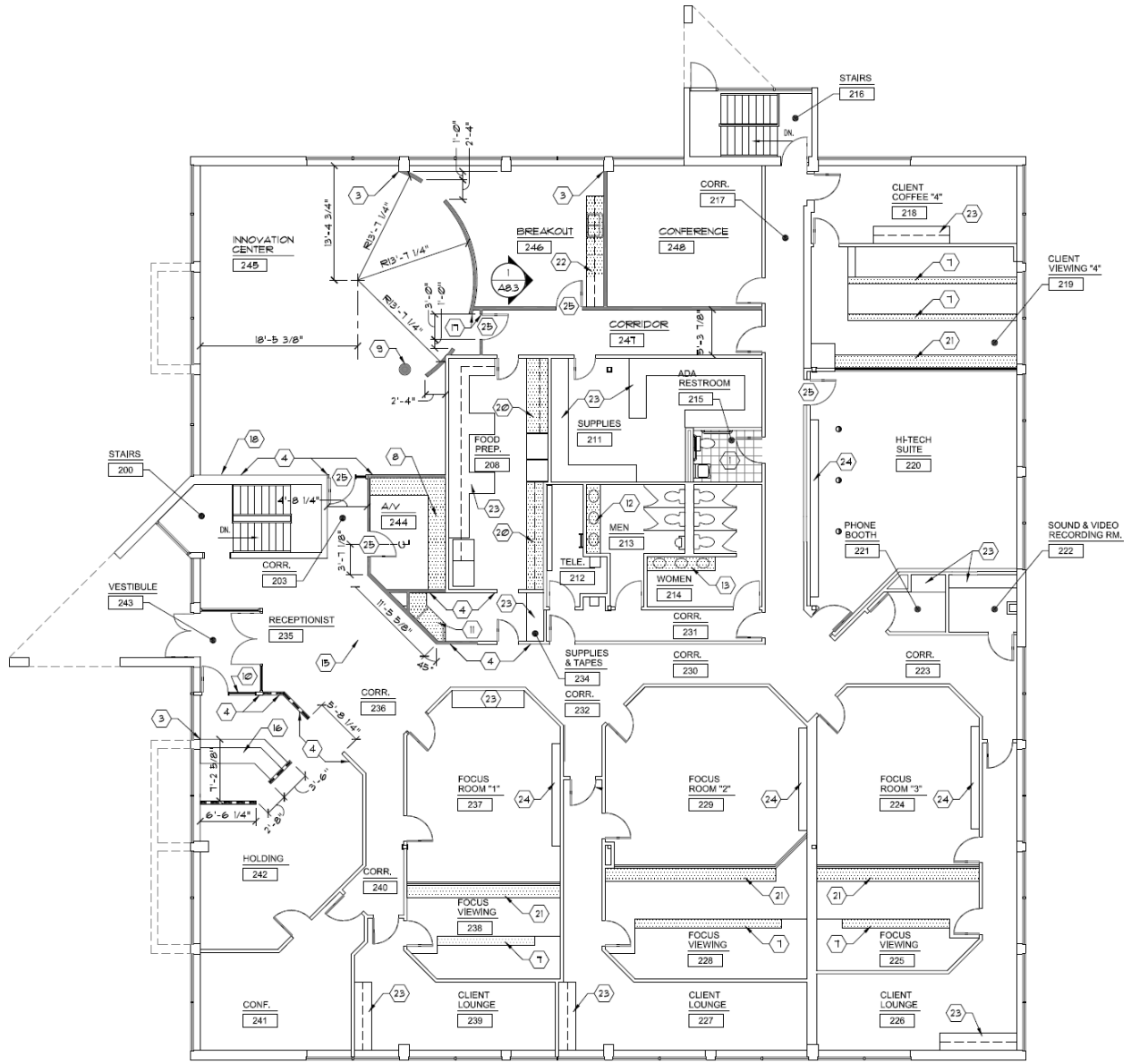
2 A2.1 SECOND FLOOR ARCHITECTURAL PLAN SCALE: 1/8" = 1'-0" N
