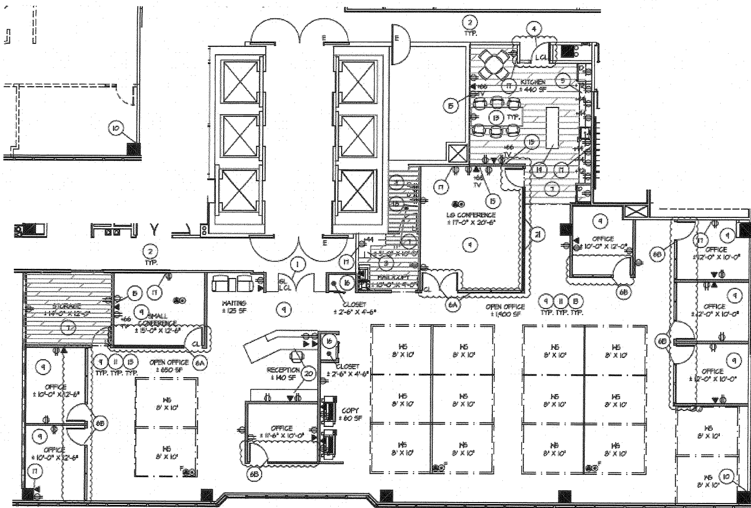
○ SUITE 750 - NEW FLOOR PLAN
