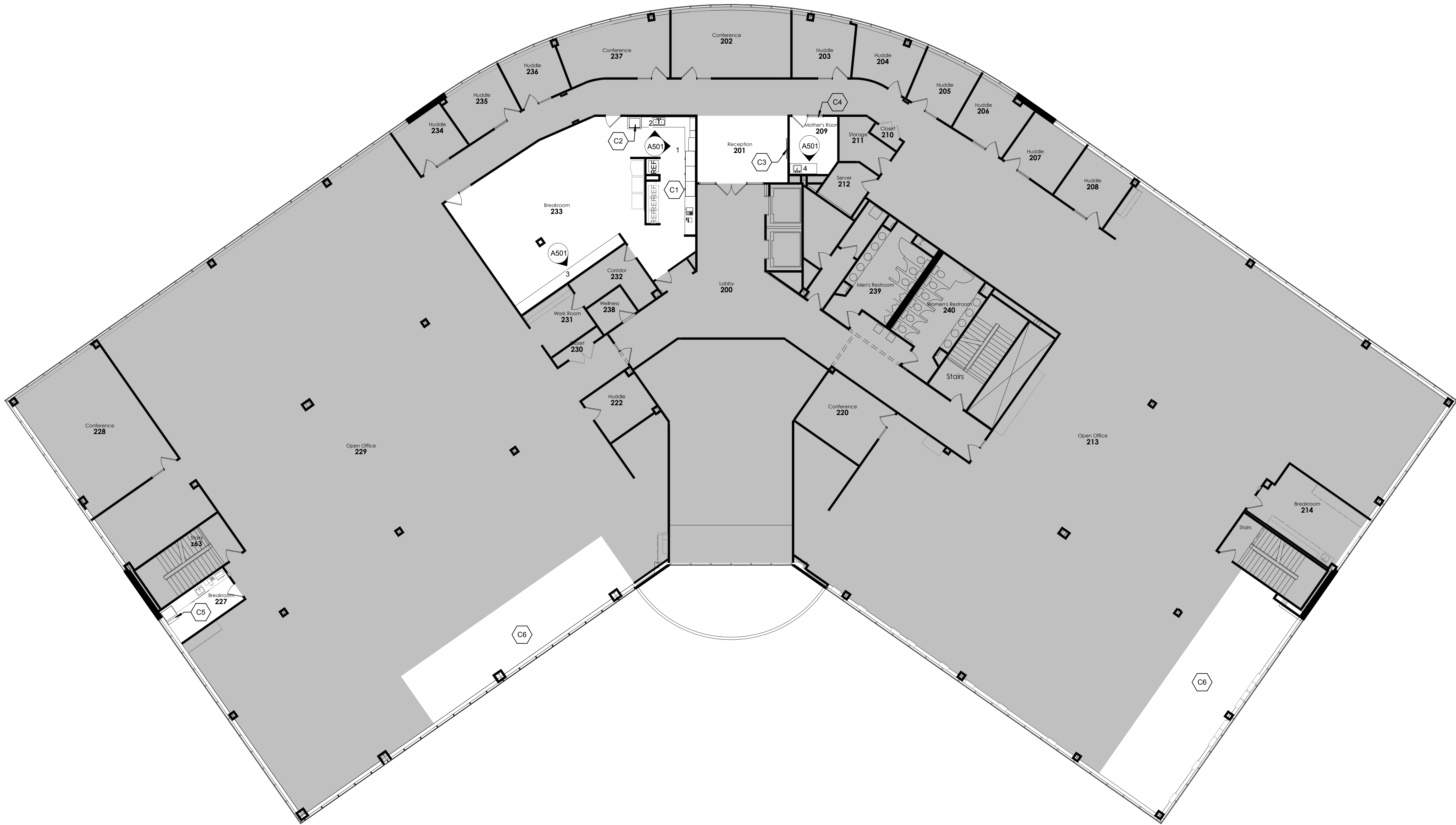
1 LEVEL 2 CONSTRUCTION FLOOR PLAN 3/32" = 1'-0"
