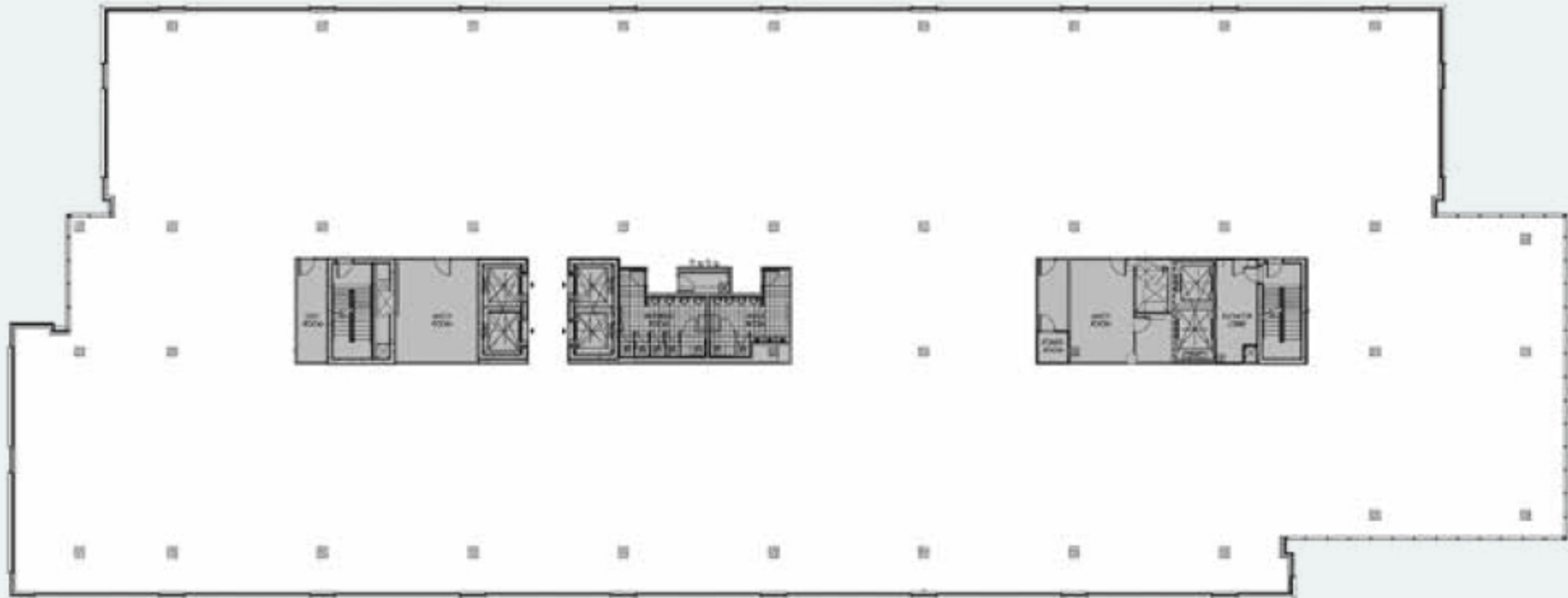
TYPICAL FLOOR PLAN 32,288 SF
