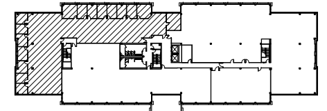
3rd FLOOR KEY PLAN
