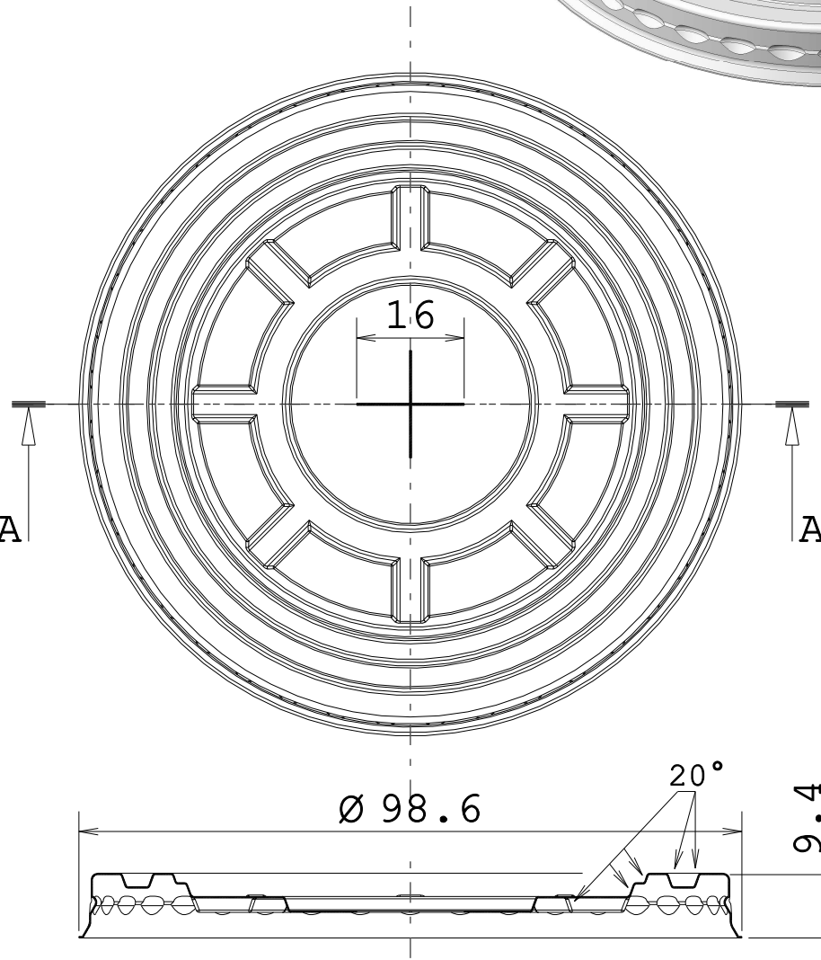
Sect. A-A
