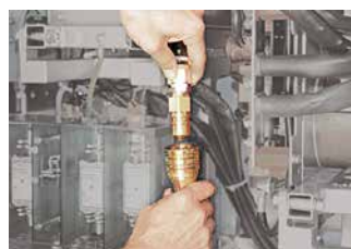
Liquid cooling can be disconnected quickly and without any spilling using quick-release couplings.
