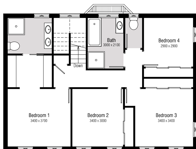
UPPER FLOOR LAYOUT
